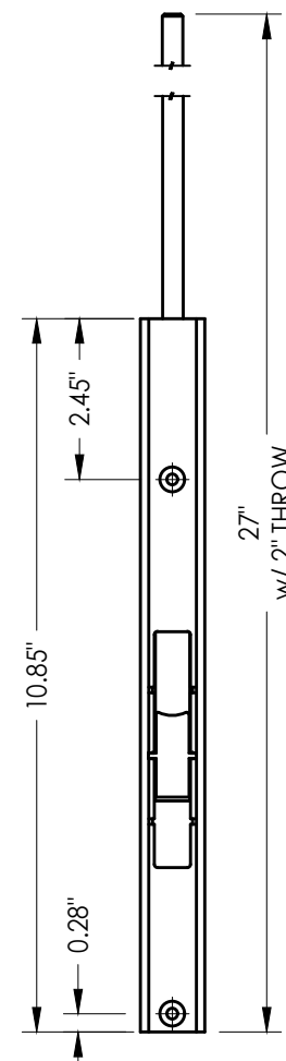
D SLIDE LOCK FLUSHBOLT ASSEMBLY HURRICANE ASTRAGAL
