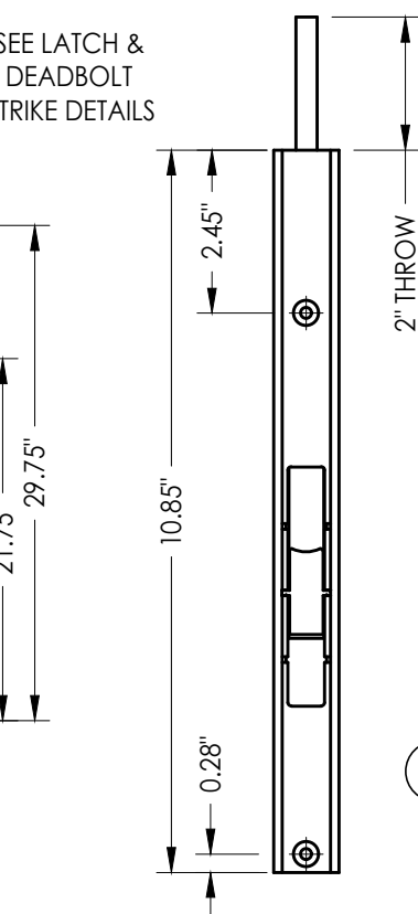
SLIDE LOCK FLUSHBOLT ASSEMBLY STANDARD ASTRAGAL
