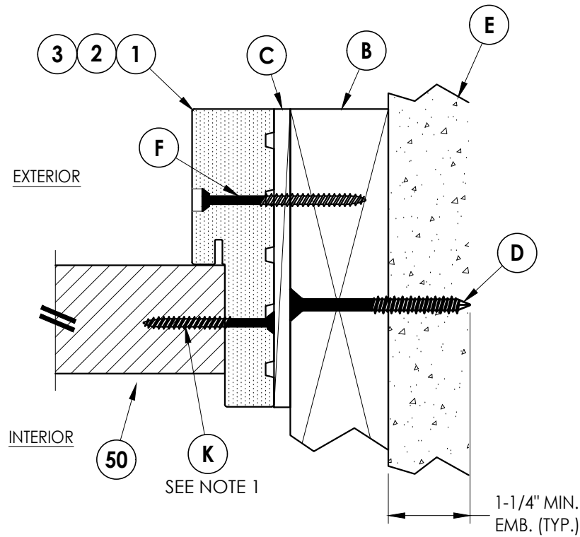
2 HORIZONTAL CROSS SECTION 5 Inswing Shown (Outswing Similar) 2X Buck Construction
